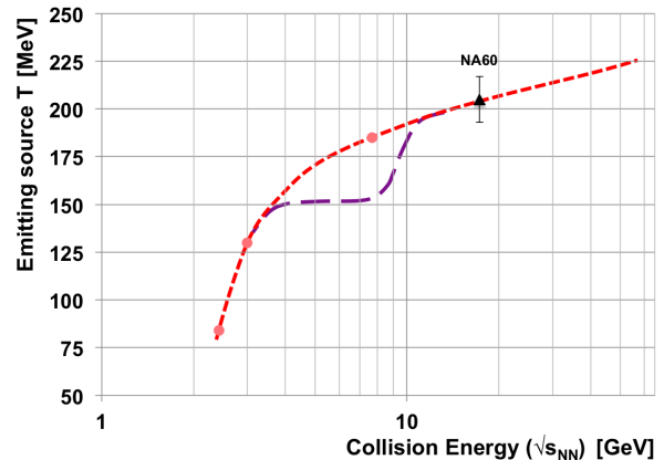
FIG. 10. Excitation function of the fireball temperature T extracted from intermediate dilepton mass distributions as calculated with a coarse-graining approach (dotted red curve) [54]. The dashed violet curve corresponds to a speculated shape with phase transition occurring in the SIS100 energy range. The black triangle corresponds to the temperature as measured by the NA60 collaboration at SPS [56].
