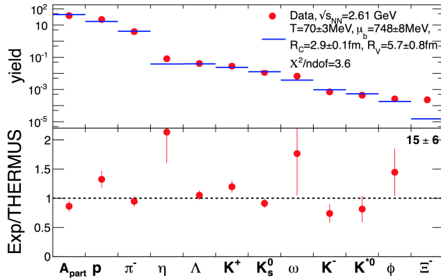
FIG. 8. Yield of hadrons measured in Ar + KCl collisions at an energy of 1.76A GeV by the HADES collaboration (full symbols). The horizontal bars represent a fit by a thermo-statistical model [48].
