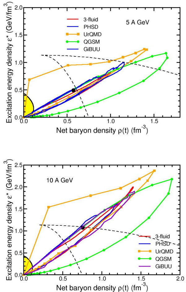
FIG. 2. Time evolution of the excitation energy density \epsilon^* and the net-baryon density \rho in the center of the fireball for central Au+Au collisions at beam energies of 5A GeV (upper panel) and 10A GeV (lower panel) calculated by various transport codes and a hydrodynamic model [12, 13]. The excitation energy density is defined as \epsilon^* = \epsilon - m_N \rho (see text). The full symbols on the curves for UrQMD and QGSM indicate time steps of 1 fm/c. The dashed lines enclose the regions of phase coexistence.
