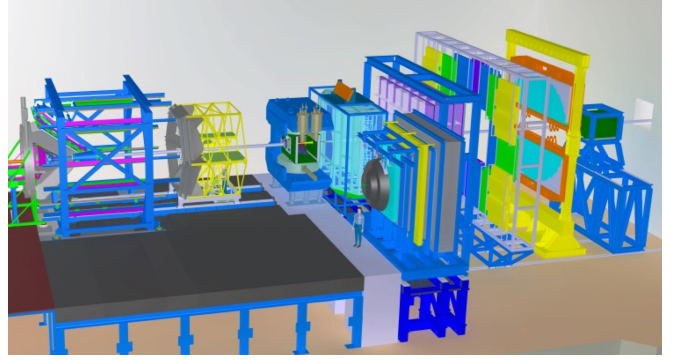
FIG. 4. The CBM experimental setup together with the HADES detector (left). Each setup has its own target. During HADES operation, the beam will be stopped by a beam dump in front of CBM. The CBM components are described in the text. For muon measurements, the RICH will be exchanged by the MuCh which is shown in a parking position to the right of the beam axis.
