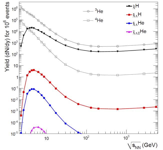
FIG. 11. Energy dependence of hypernuclei yields at midrapidity for 10^6 central collisions as calculated with a thermal model. The predicted yields of {}^3\text{He} and {}^4\text{He} nuclei are included for comparison [63].
