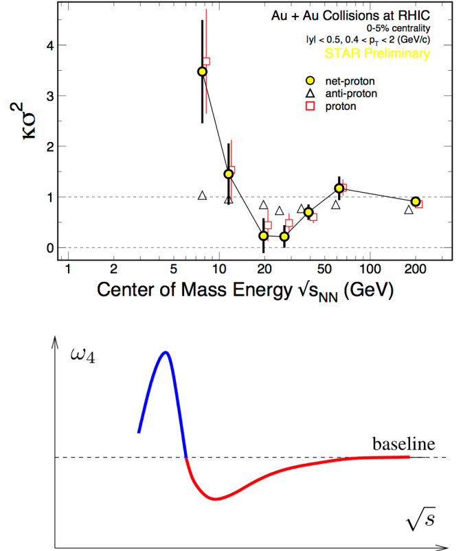
FIG. 7. Upper plot: Energy dependence of the product of moments \kappa\sigma^2 (kurtosis times squared standard deviation) of the net-proton multiplicity distribution (yellow circles) for top 0-5% central Au+Au collisions. The Poisson expectation is denoted as dotted line at \kappa\sigma^2 = 1 [36, 37]. Lower plot: Net-baryon 4th moment \omega_4 = C_4/(N_b - N_{\bar{b}}) as a function of collision energy. C_4 is the 4 th order cumulant, N_b is the number of baryons and N_{\bar{b}} the number of antibaryons. When the system is near the critical point, the 4th moment is expected to deviate from the base line. The curve is based on a calculation [42] by converting the Ising-reduced temperature t(T, \mu_B) into collision energy \sqrt{s} .
