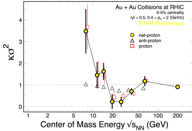
FIG. 7. Upper plot: Energy dependence of the product of moments \kappa\sigma^2 (excess kurtosis times variance squared standard deviation) of the net-proton multiplicity distribution (yellow circles) for top 0-5% central Au+Au collisions. The Poisson expectation is denoted as dotted line at \kappa\sigma^2 = 1 [37, 38]. Lower plot: Net-baryon 4th moment \omega_4 = C_4/(N_b - N_{\bar{b}}) as a function of collision energy. C_4 is the 4 th order cumulant, N_b is the number of baryons and N_{\bar{b}} the number of antibaryons. When the system is near the critical point, the 4th moment is expected to deviate from the base line. The curve is based on a calculation [43] by converting the Ising-reduced temperature t(T, \mu_B) into collision energy.
