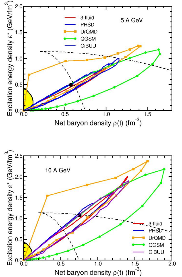
FIG. 2. Time evolution of the excitation energy density \epsilon^* versus the net-baryon density \rho in the center of the fireball for central Au+Au collisions at beam energies of 5A GeV (upper panel) and 10A GeV (lower panel) calculated by various transport codes and a hydrodynamic model [12, 13]. The excitation energy density is defined as \epsilon^* = \epsilon - m_N \rho (see text). The full symbols on the curves for UrQMD and QGSM indicate time steps of 1 fm/c. The dashed lines enclose the regions of phase coexistence [14]. The yellow zone denotes post-freezeout streaming.
