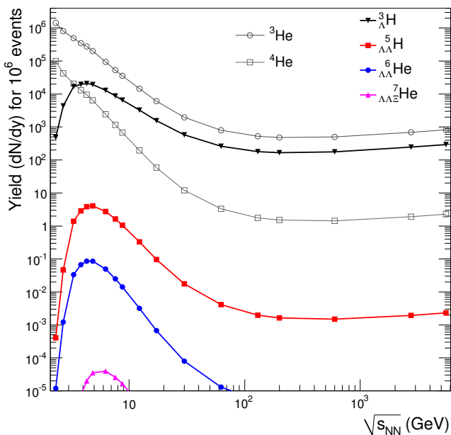
Fig. 11. Energy dependence of hypernuclei yields at midrapidity for 10^6 central collisions as calculated with a thermal model. The predicted yields of ^3\text{He} and ^4\text{He} nuclei are included for comparison [96].
