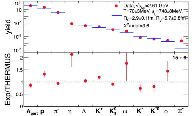
Fig. 8. Yield of hadrons measured in Ar + KCl collisions at an energy of 1.76A GeV by the HADES collaboration (full symbols). The horizontal bars represent a fit by a thermo-statistical model [66].
