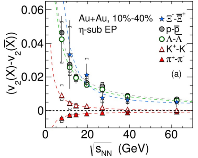
Fig. 6. The difference in elliptic flow between particles and their corresponding antiparticles (see legend) as a function of \sqrt{s_{NN}} for 10% - 40% central Au+Au collisions as measured by the STAR collaboration at RHIC [19]. The systematic errors are indicated by the brackets. The dashed lines in the plot are fits with a power-law.
