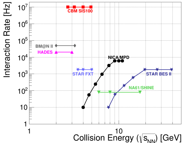
Fig. 3. Interaction rates achieved by existing and planned heavy-ion experiments as a function of center-of-mass energy [20, 22, 23, 24]. “STAR FXT” denotes the fixed-target operation of STAR. High-rate experiments are also proposed at JPARC [25] and at SPS [26], but these are still in a conceptual stage.
